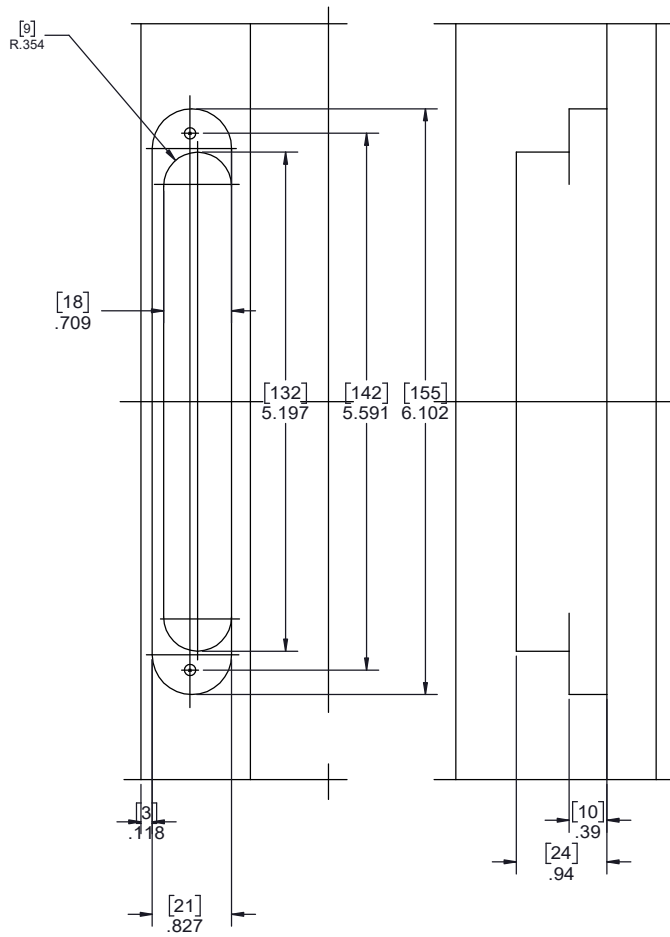
Milling Frame
